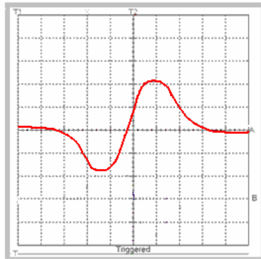
SHORT-CIRCUITED COIL
