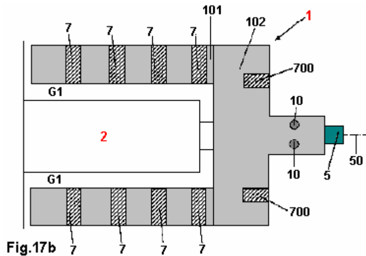
Fig17b is a schematic view of one rotor drum and part of the inner stator 2, where the view is perpendicular to the shaft axis 50. The rotor 1 is clamped to the shaft 5 by the screws 10 and held rigidly in position. The shaft 5 passes through a ball bearing inset into the inner stator 2 and so can rotate freely relative to the inner stator. The rotor has two drum, or bell-shaped, sections which surround the inner stator. The rotor 1 has a hollow cylindrical section 101, which extends away from the top surface 102. Since the inner stator is fixed and prevented from rotation by it's anchoring device (component 4 in Fig.1), the rotor spins the hollow cylinder 101 around it. The hollow cylinder 101 of rotor 1 is separated from the inner stator 2 by an annular air gap G1. The hollow cylinder 101 of rotor 1 has magnets 7 sunk into holes in it. The top surface 102 of the rotor 1 also has holes in it and these are used to install the magnets 700 in it.
