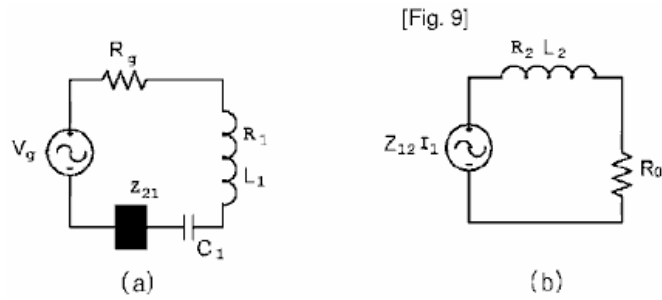
Fig.9A and Fig.9B are equivalent circuit diagrams of the primary and secondary sides in the equivalent circuit of Fig.8 .
