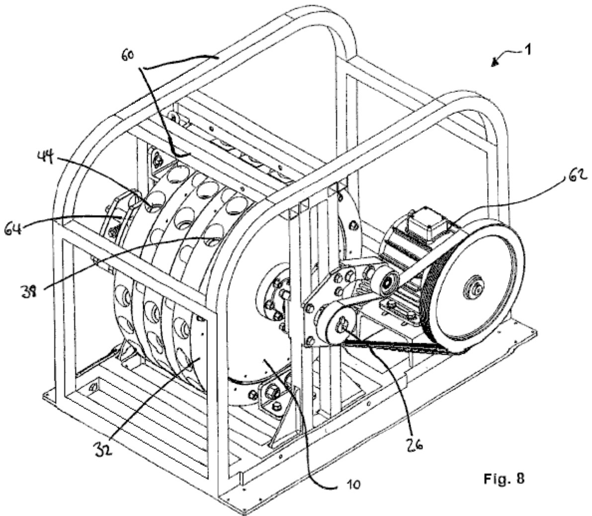
Fig.8 is a perspective view showing one embodiment of the magnetic repellant motor coupled to an electrical generator.
