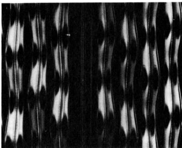
Fig. 506. Microphotographs of grooves in 45/45 stereo records. (Westrex Corp.)
