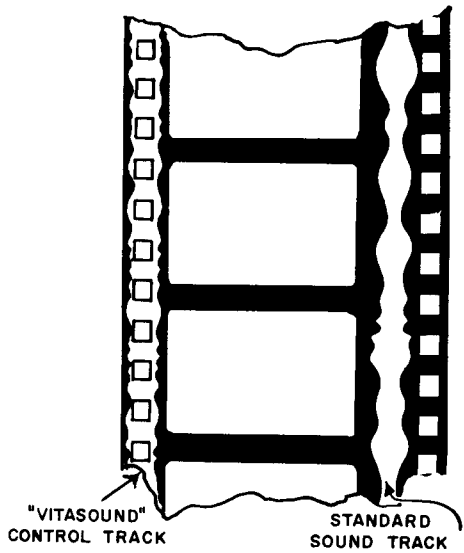
Fig. 305. The "Vitasound" system developed by Warner Brothers.
