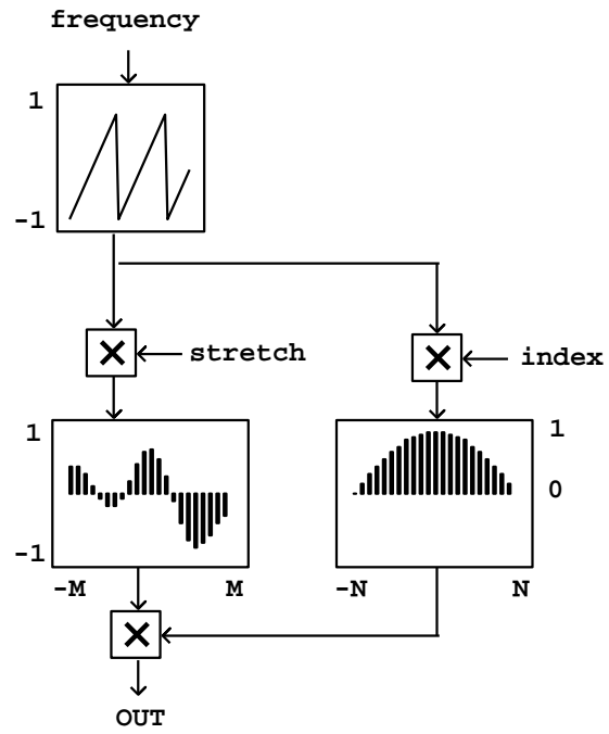
Figure 6.3: Wavelable synthesis generalized as a variable spectrum generator.
