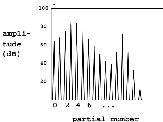
Figure 6.12: Spectrum from a two-formant PAF generator.
