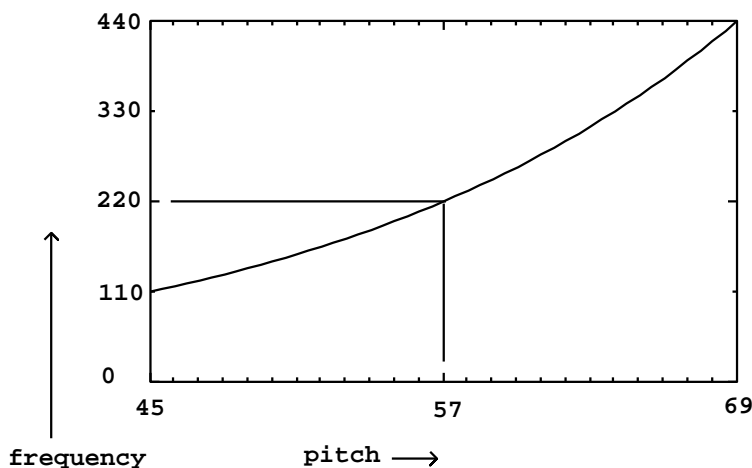
Figure 1.4: The relationship between “MIDI” pitch and frequency in cycles per second (Hertz). The span of 24 MIDI values on the horizontal axis represents two octaves, over which the frequency increases by a factor of four.
