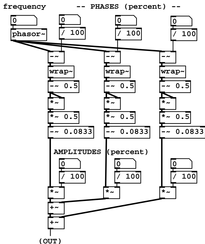
Figure 10.13: Combining parabolic waves to make a waveform with three corners.
