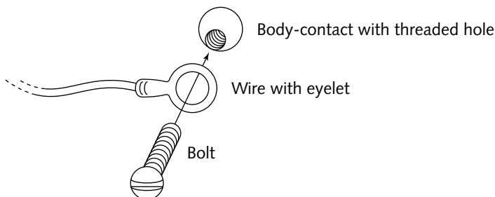
FIGURE 12-9: Wire-to-body-contact
