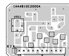
HIC Board (SIDE:B)
